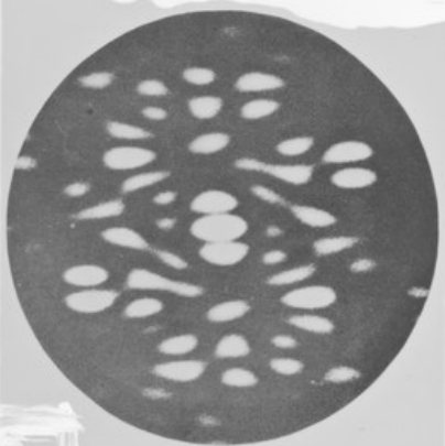
2 Optical transform of two centrosymmetrically- related units equivalent to the real part of the transform shown in 1
