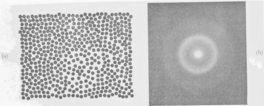
Optical diffraction pattern of a two-dimensional structure showing "liquid" interferences.
