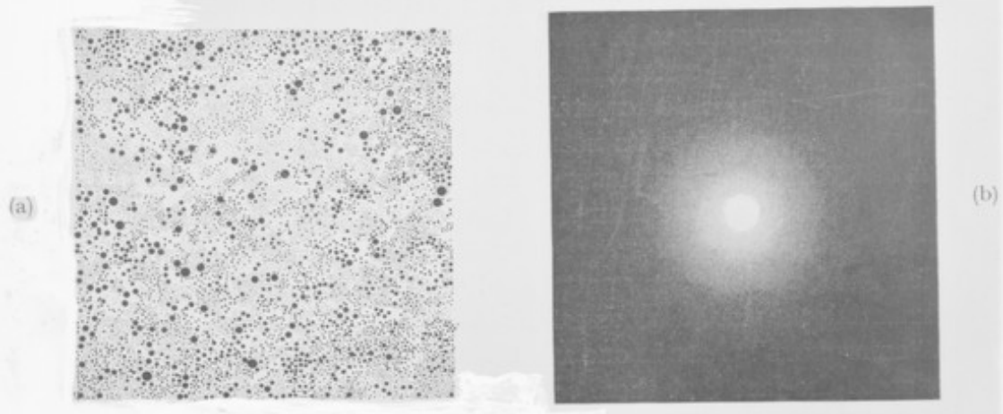
Optical diffraction pattern of a structure showing "gas" interferences.
