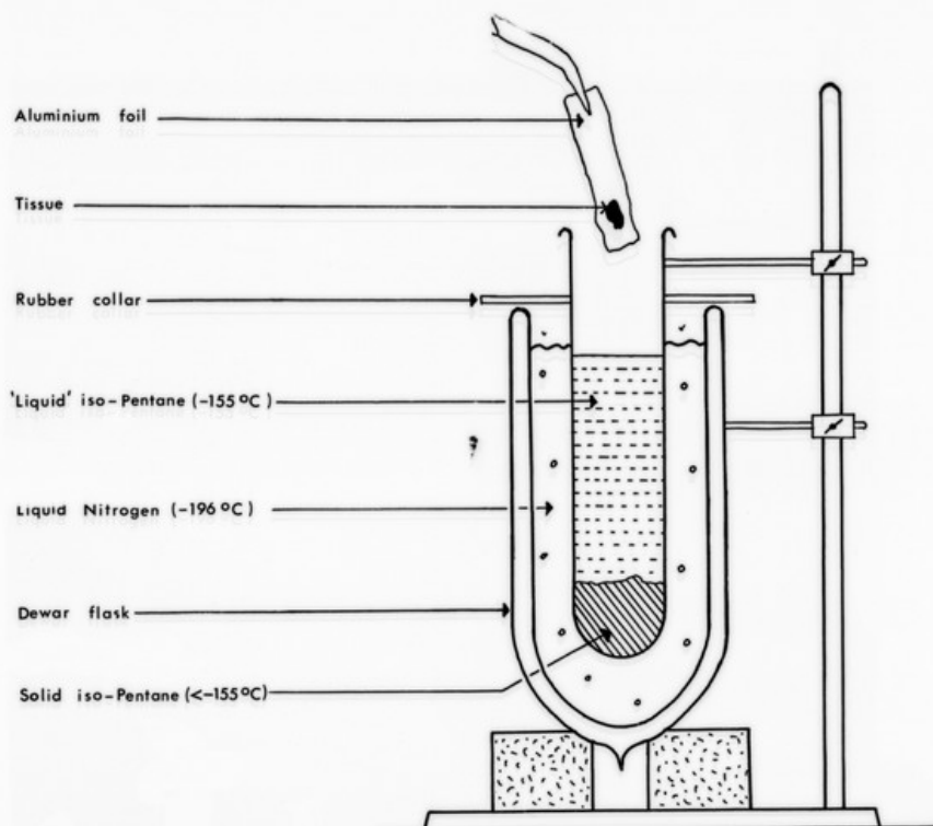
Fig.2 FREEZING APPARATUS
