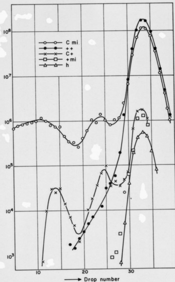
Cross \lambda cmi C^{13}N^{15} \times \lambda ++ C^{12}N^{14} . Titer of the progeny phages of different genotypes in the drops collected after centrifugation. \lambda h was added as density and band shape reference.
