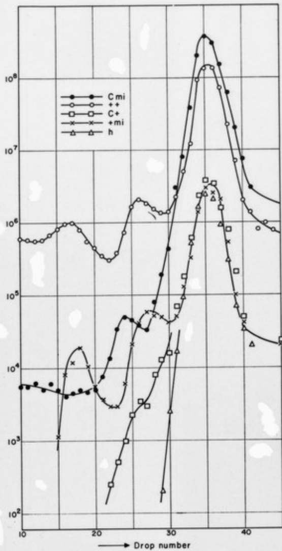
Cross \lambda^{++} C^{15}N^{14} \times \lambda_{emi} C^{15}N^{14} . Titer of the progeny phages of different genotypes in the drops collected after centrifugation. \lambda_h was added as density and band shape reference.
