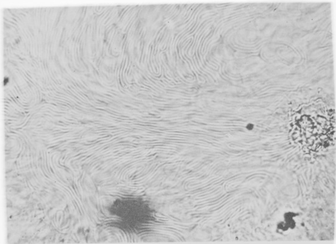
12. Periodic lines in solution of DNA in 0.1 M NaCl. S \approx 1 \mu . Cell thickness 0.1 m Natural light.
