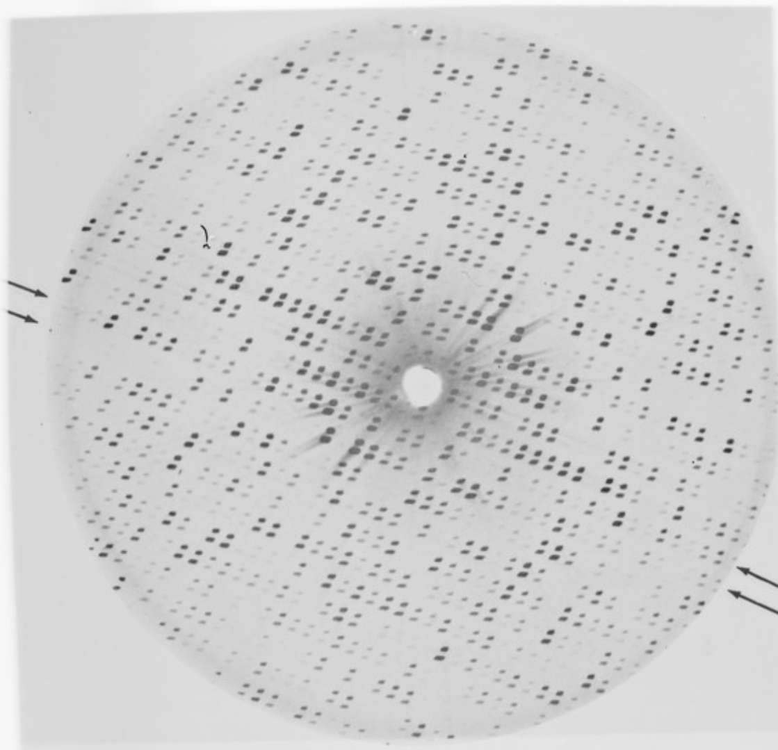
Comparison of the X-ray diffraction patterns of azide metmyoglobin and of the native protein. The photographs are superposed, with the azide pattern above. These photographs contain the h0l reflexions to a spacing corresponding to 2.8 Å resolution.
