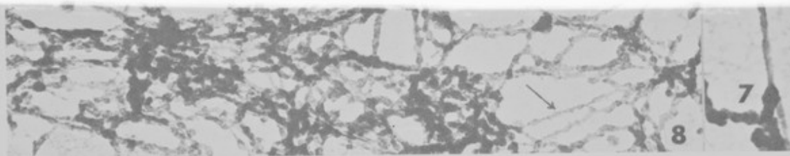
FIGURE 6. Chromosome microfilaments spread on a water surface, fixed in 1% tannic acid and dried from 100% ethanol. The microfilaments are coiled, and consist of two subunits
