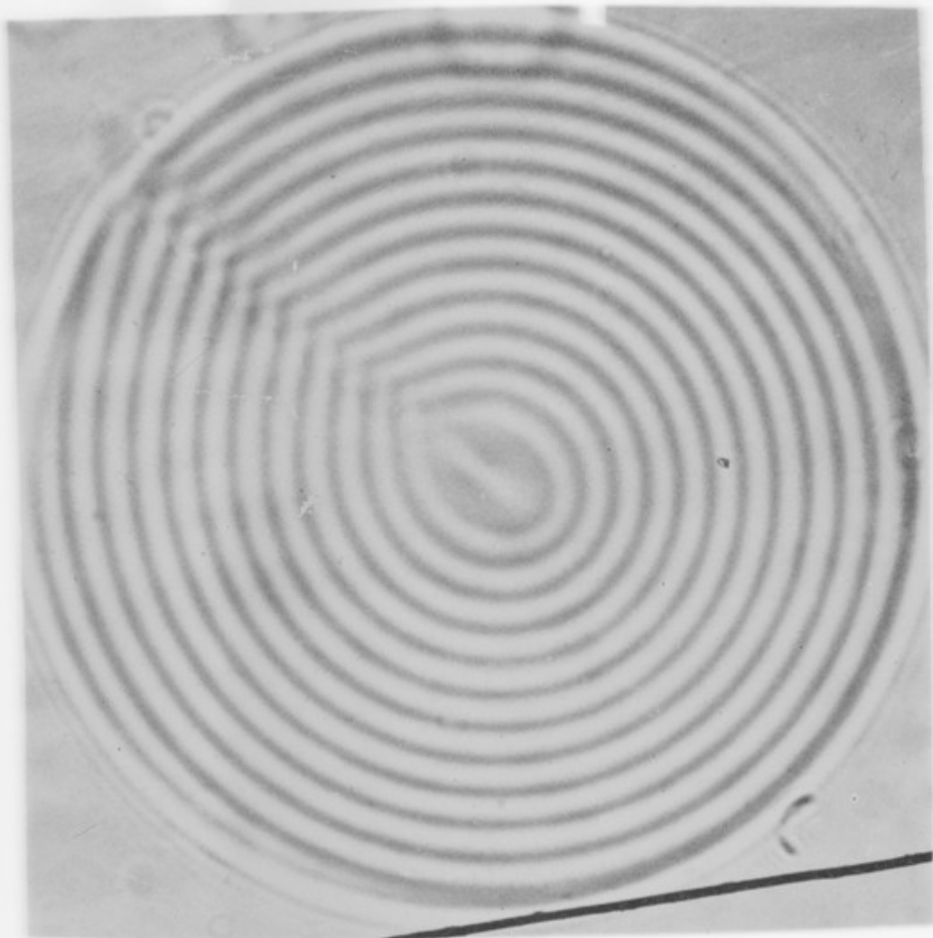
spherulite
