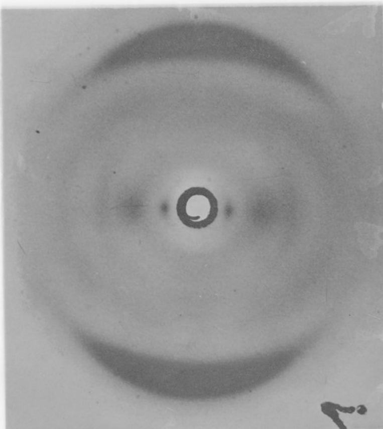
PLATE I. X-ray diffraction pattern given by the complex of Li DNA with proflavine at 75% relative humidity.
