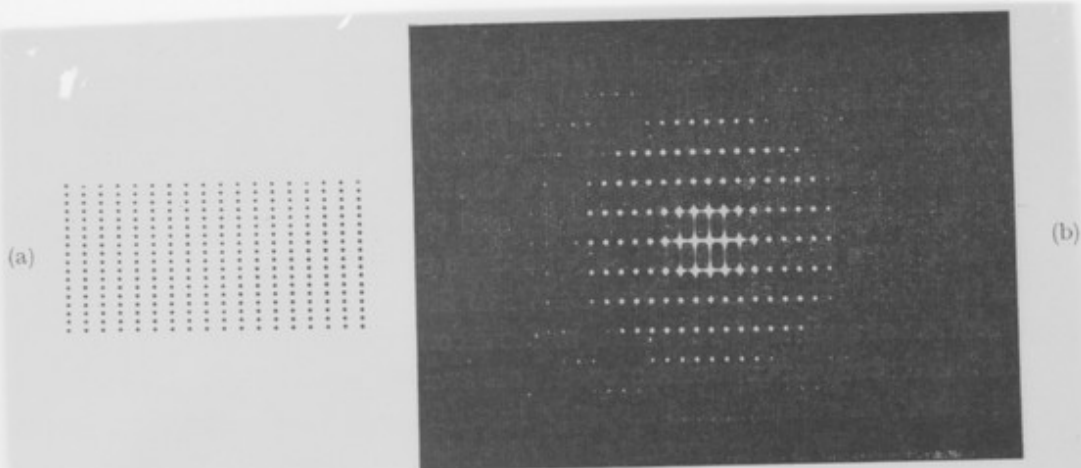
Fig. 1 Optical diffraction pattern of a two-dimensional model of a "perfect crystal". (a) Negative of the model; (b) Fraunhofer's diffraction of (a).
