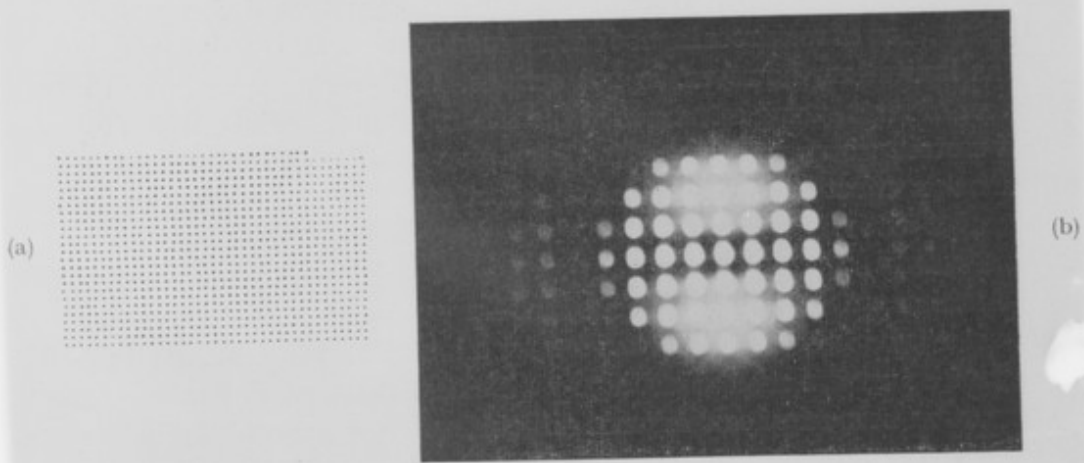
Fig. 2 Optical diffraction pattern of a two-dimensional lattice showing "frozen thermal distortions".
