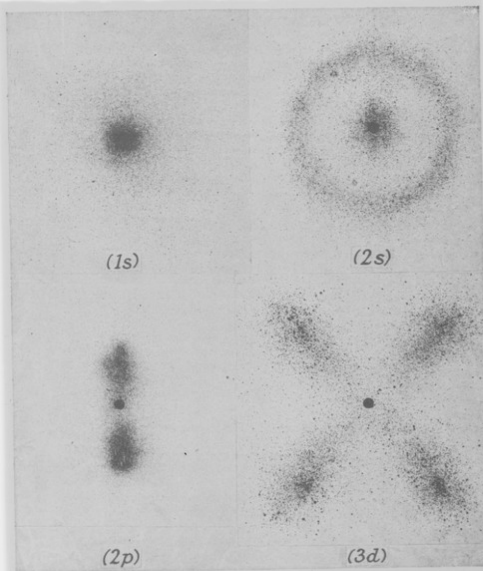
Some atomic orbitals for hydrogen.
