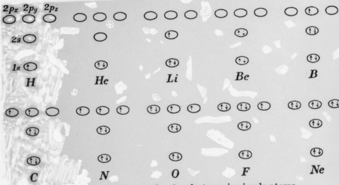
Cell diagrams for the electrons in simple atoms.
