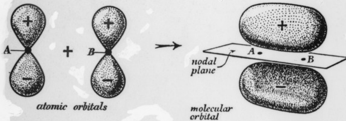
Formation of a \pi -type bonding molecular orbital.
