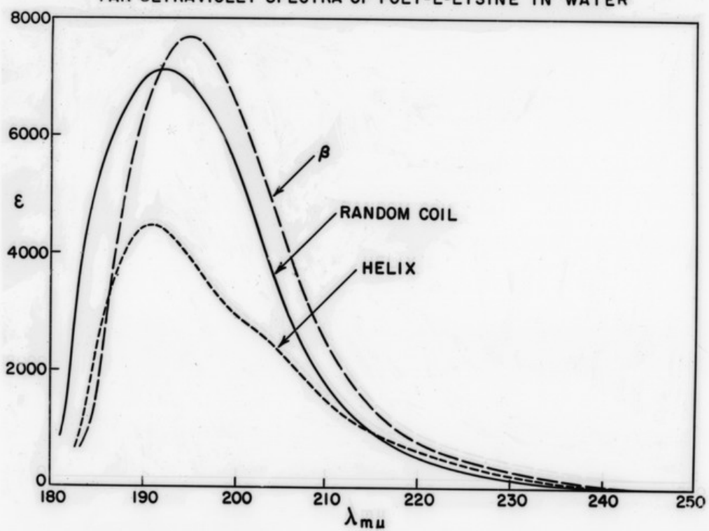
FAR ULTRAVIOLET SPECTRA OF POLY-L-LYSINE IN WATER
