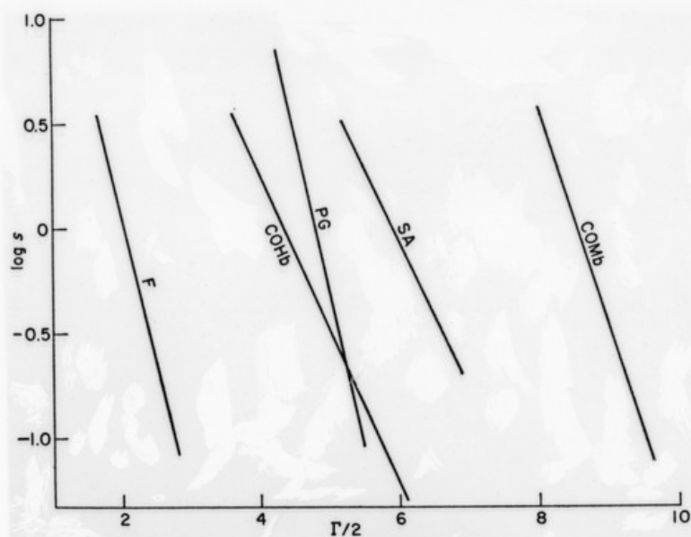
Relation between \log s and ionic strength of ammonium sulfate for several proteins. From Cohn and Edsall (1943). F = fibrinogen; COHb = carboxyhemoglobin; PG = pseudoglobulin; SA = serum albumin; COMb = carboxymyoglobin.
