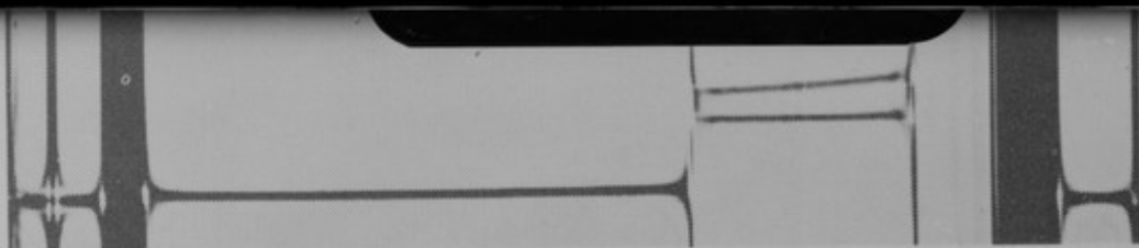
Sedimentation equilibrium study of sucrose with short liquid column, showing both Rayleigh fringe and schlieren patterns
