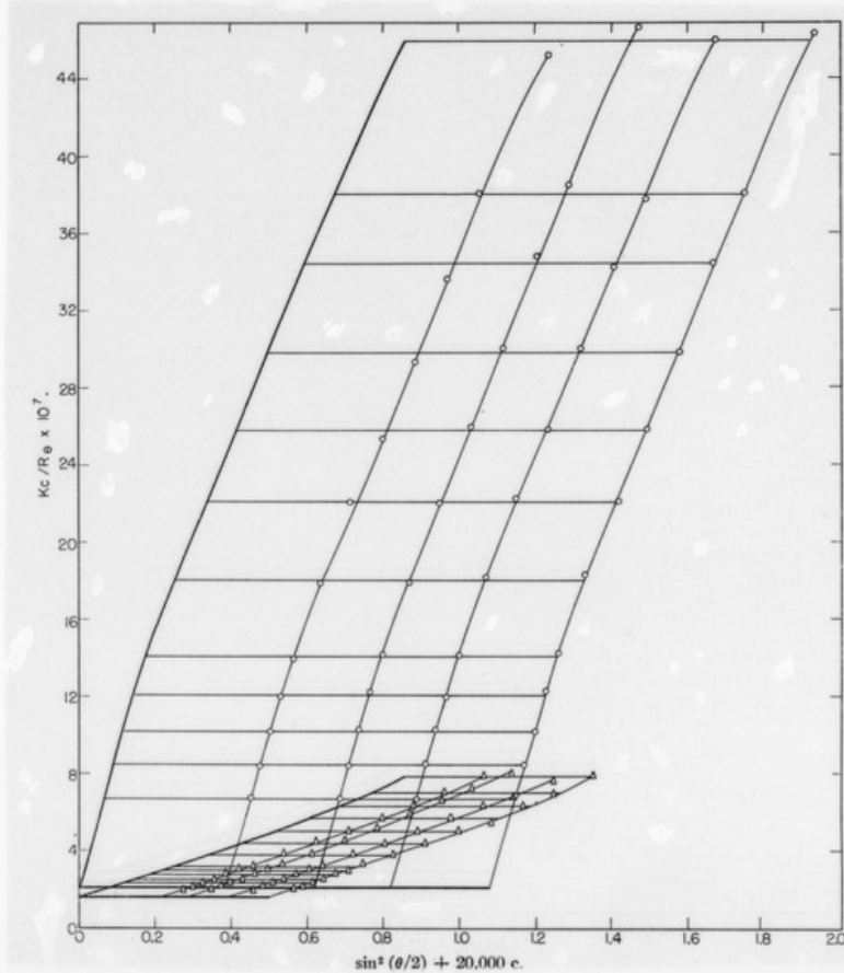
Fig. 2.—Light scattering data of DNA before (O) and after (Δ) exposure to pH 12.1 for one hour; measurements made at pH 7; ionic strength 0.165.
