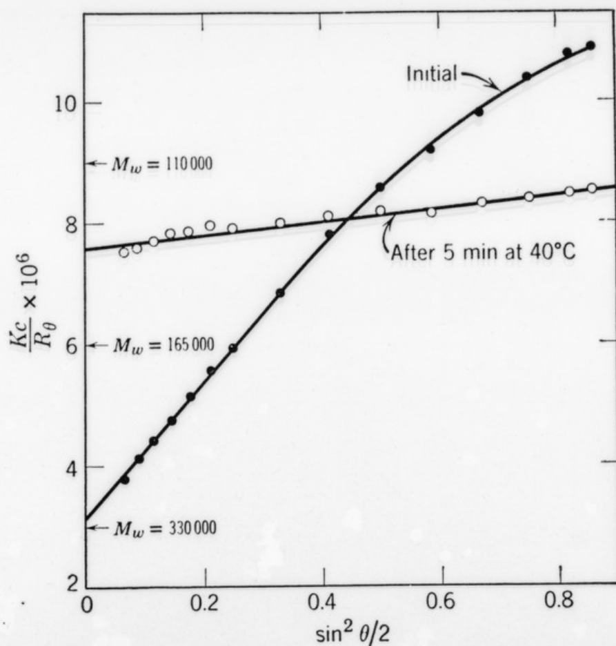
FIG. 6. Denaturation of collagen in solutions. ● = before denaturation; ○ = after denaturation.
