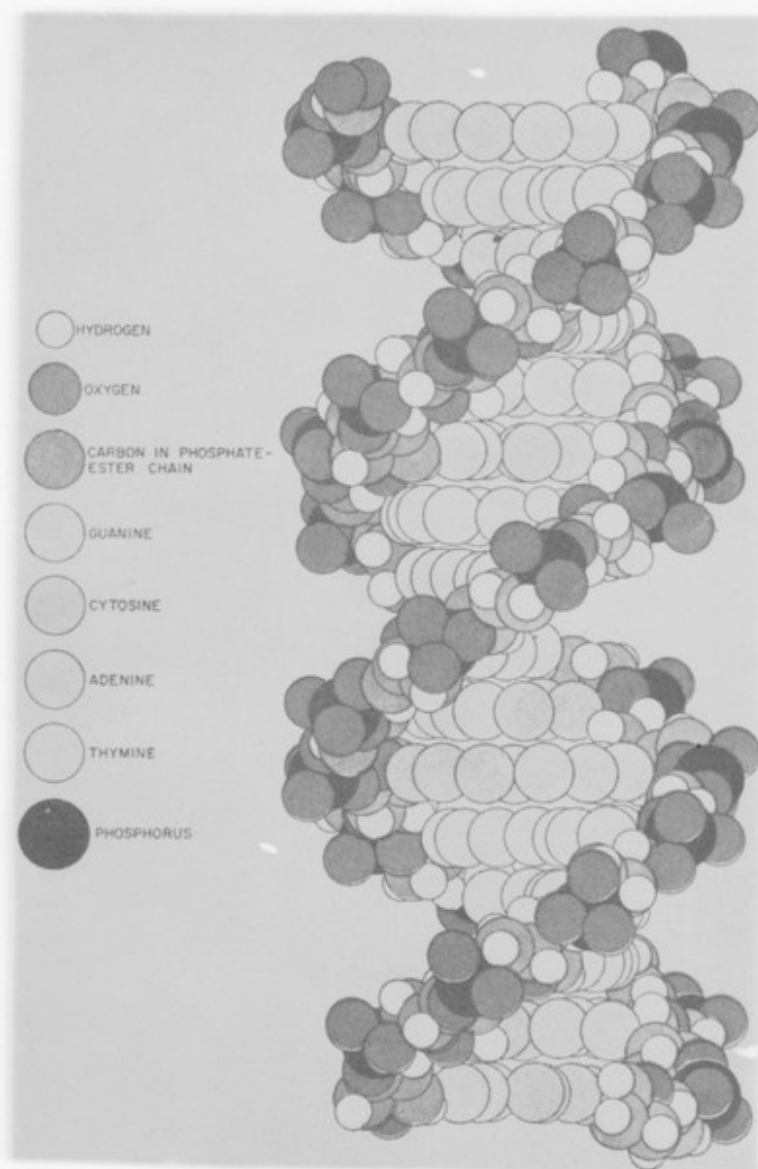
FIG. 2. A drawing of the deoxyribonucleic acid molecule, using circles to represent the atoms. Taken from Feaghtman et al. , Nature 175, 854 (1955).
