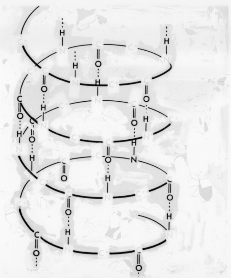
Fig. 4.8b. The \alpha -helix (schematic).
