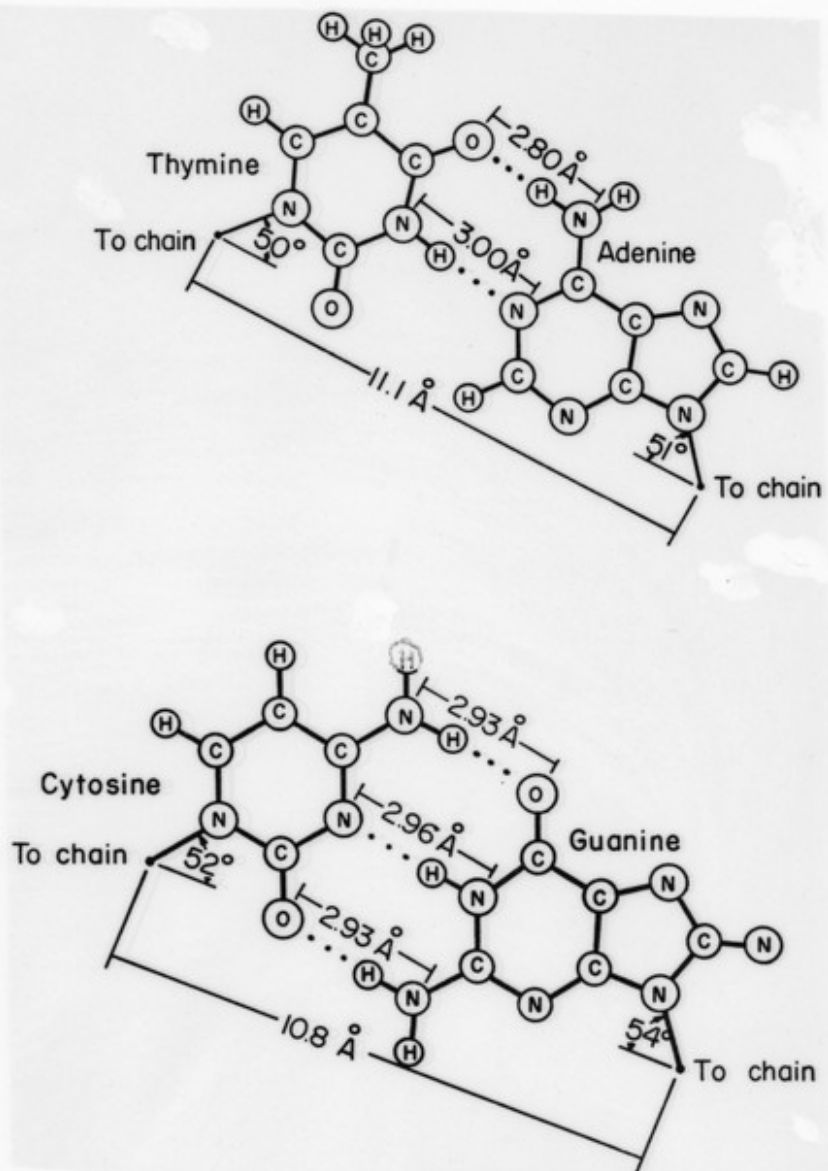
FIG. 3. The hydrogen bonding of the base pairs occurring in deoxyribonucleic acid. Taken from Pauling and Corey, Arch. Biochem. Biophys. 65, 164 (1956)
