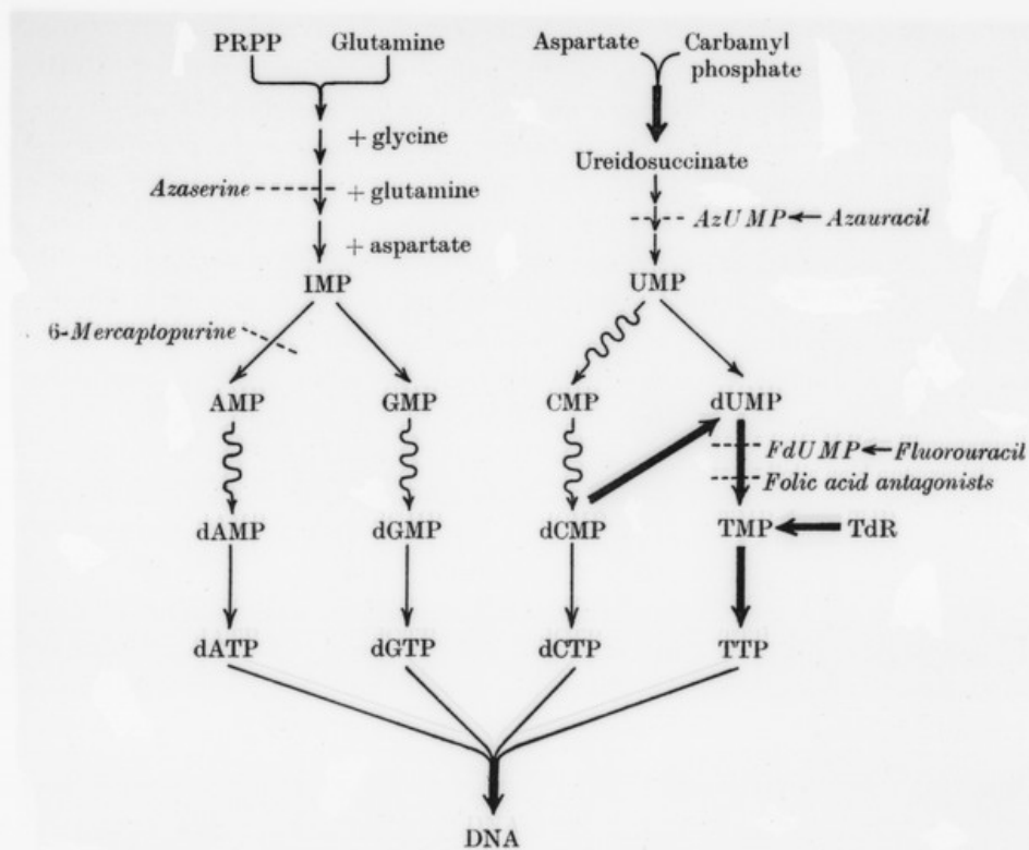
Pathway of DNA biosynthesis. Undulating arrows denote that the level of phosphorylation has not been taken into account. Heavy arrows denote reactions which are increased in rapidly growing tissues such as regenerating rat liver. The action of some inhibiting agents is indicated.
