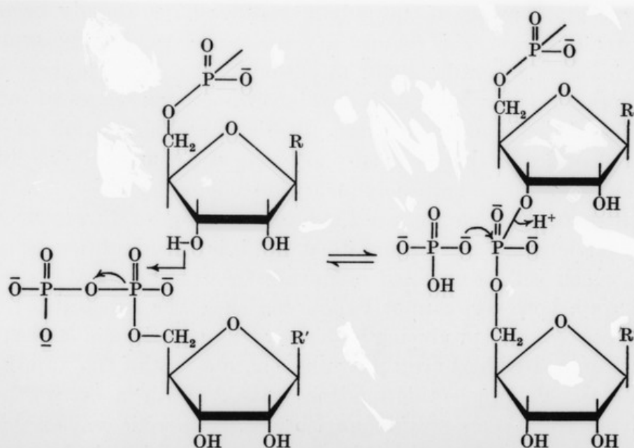
Action of polynucleotide phosphorylase (Khorana, 1960).
