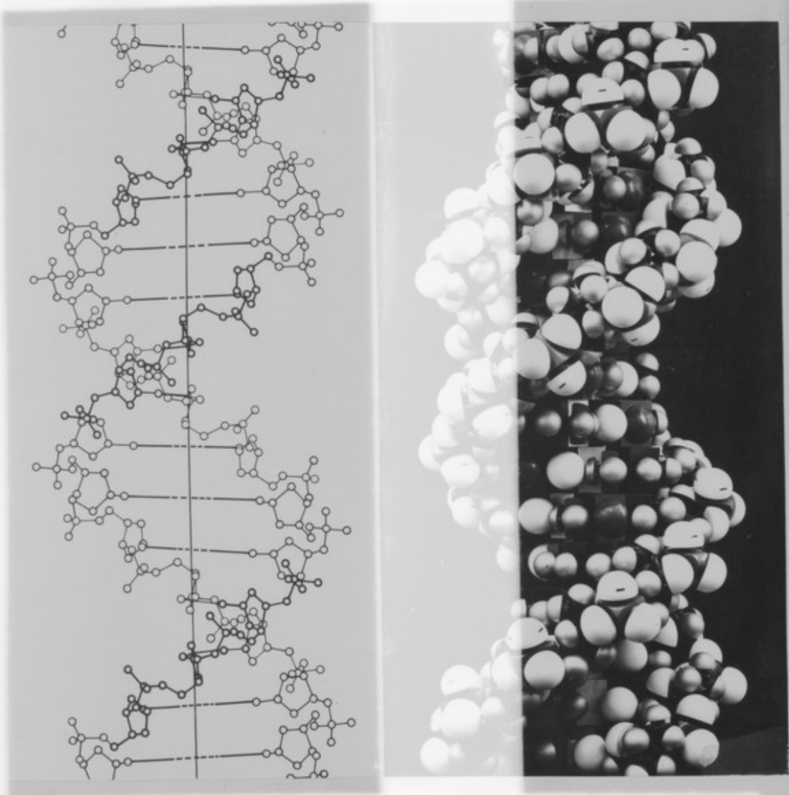
Fig. 4. Model of the B configuration of DNA.
