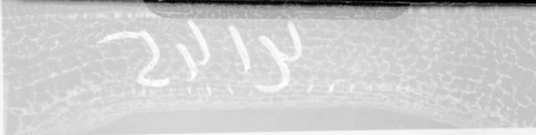
1A. Single-crystal rotation X-ray photograph, taken about the c -axis of rubidium hydrogen di-anisate (J. M. Skinner).
