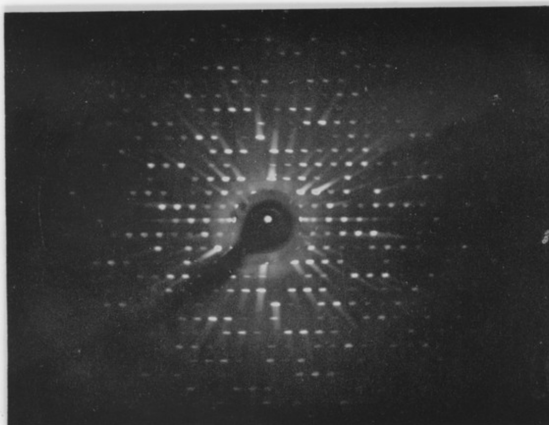
2B. Precession X-ray photograph, showing h0l reciprocal-lattice net of epi -limonol iodoacetate (Struther Arnott). (The shadow blocking off part of the net is due to the "beam catcher".)
