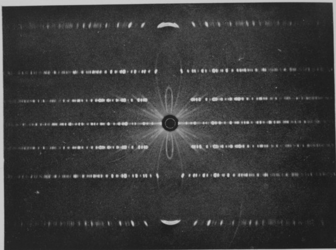
Single-crystal rotation X-ray photograph, taken about the c -axis of rubidium hydrogen di-anisate (J. M. Skinner).
