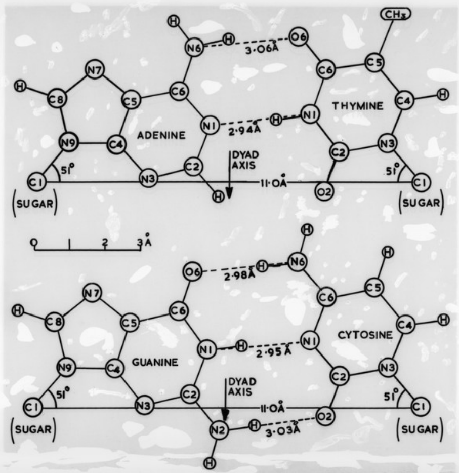
HYDROGEN BONDED WATSON-CRICK BASE PAIRS (AFTER SPENCER)
