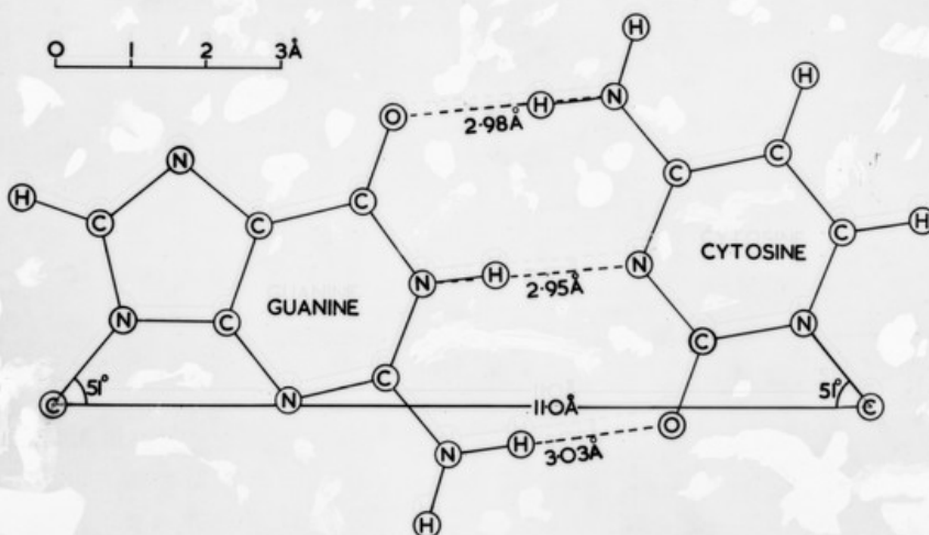
HYDROGEN BONDED WATSON-CRICK BASE PAIRS (AFTER SPENCER)
