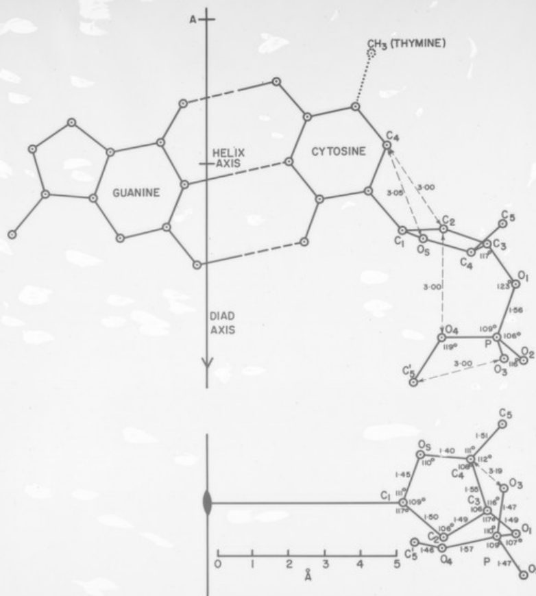
PROJECTION OF B STRUCTURE OF DNA.
