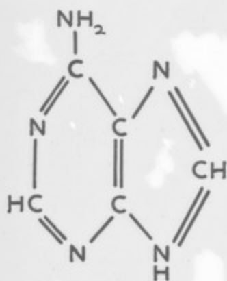
ADENINE
