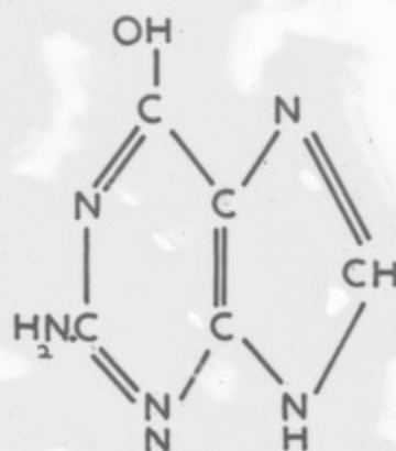
GUANINE
