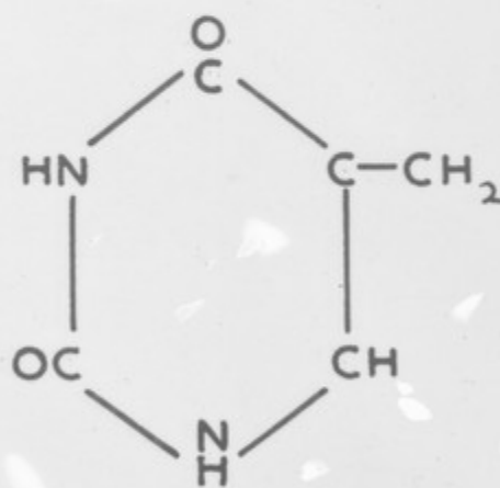
THYMINE
