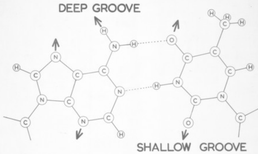
THYMINE
