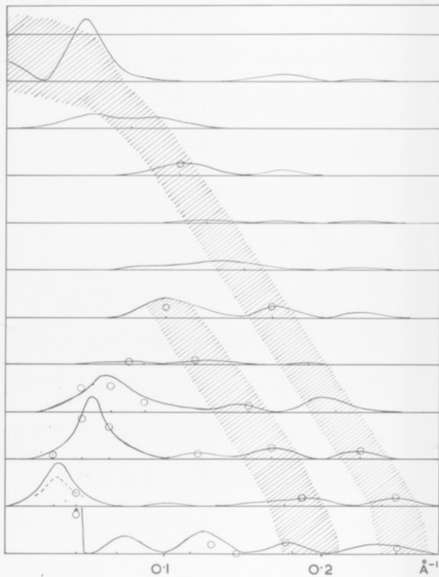
CALCULATED AND OBSERVED DIFFRACTION OF DNA (B)
