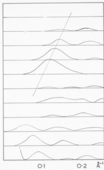
CALCULATED DIFFRACTION FROM HELICAL ARRAY OF TILTED RODS
