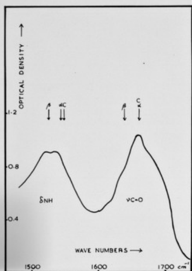
INFRA-RED SPECTRUM OF BYSSUS THREADS OF PINNA NOBILIS.
