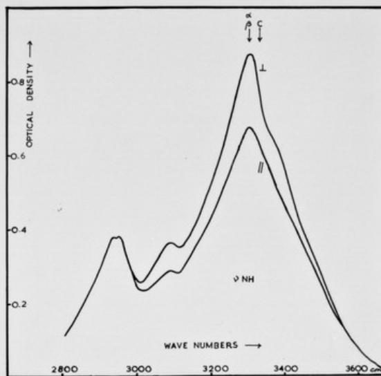
INFRA-RED SPECTRUM OF BYSSUS THREADS OF PINNA NOBILIS.
