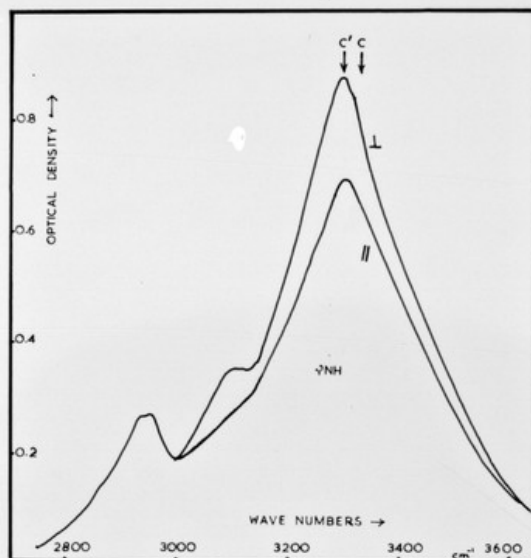
INFRA-RED SPECTRUM OF BYSSUS THREADS OF MYTILUS EDULIS.
