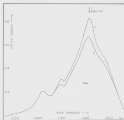
INFRA-RED SPECTRUM OF EXTRACTED COLLAGEN.
