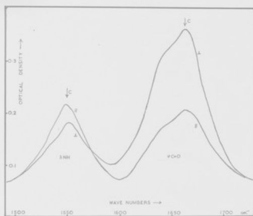
INFRA-RED SPECTRUM OF EXTRACTED COLLAGEN.
