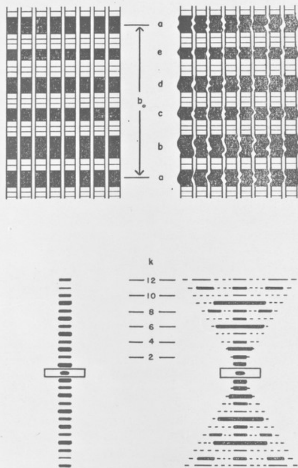
FIGURE 3.—Longitudinal sections through perfect (left) and mixed perfect and imperfect (right) models for collagen fibril structure. Eight filaments (protofibrils) are shown in each case, with the scale for filament thickness exaggerated
