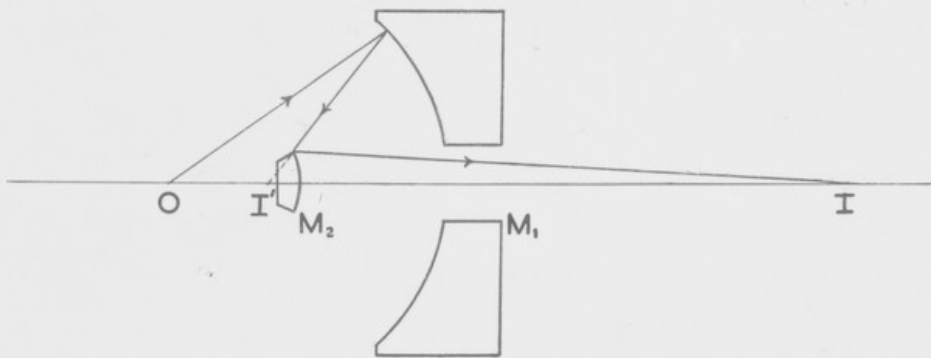
DIAGRAM OF REFLECTING OBJECTIVE
