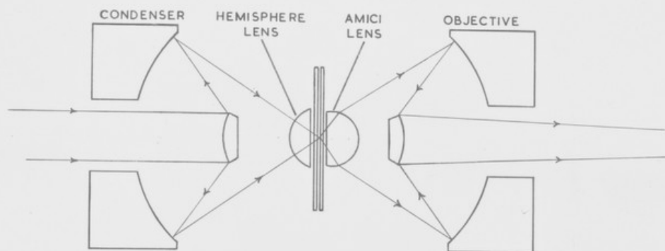
HIGH APERTURE REFLECTING OBJECTIVE
