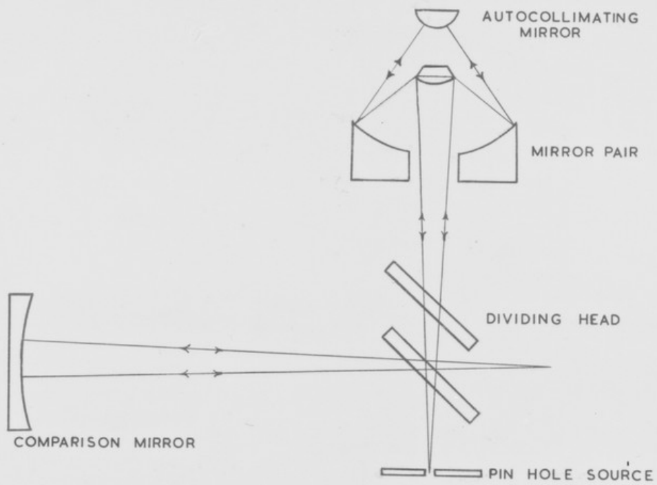
DIAGRAM OF INTERFEROMETER USED FOR TESTING REFLECTING OBJECTIVES
