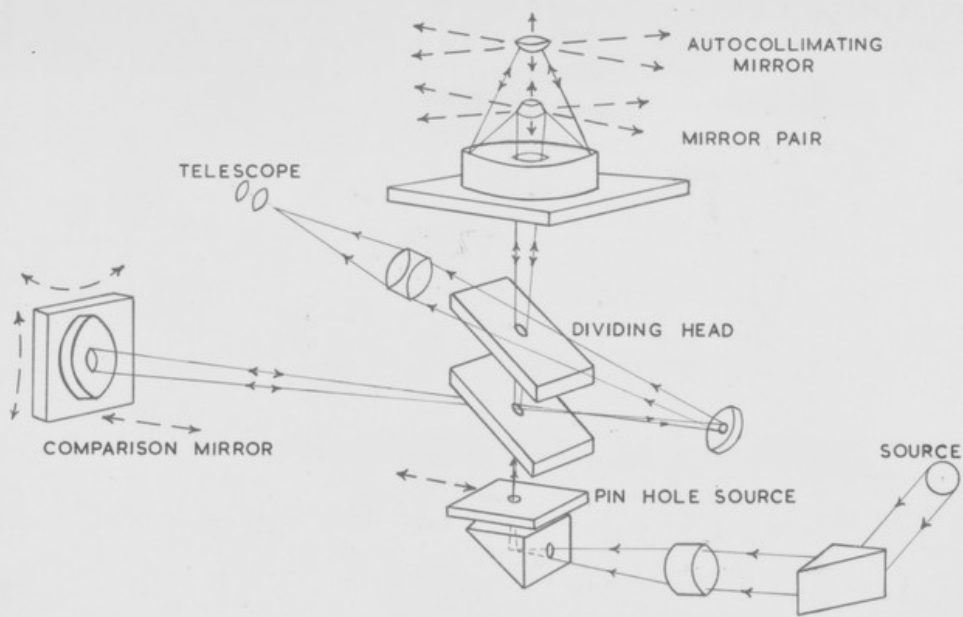
PERSPECTIVE DRAWING OF INTERFEROMETER USED FOR TESTING REFLECTING OBJECTIVES
