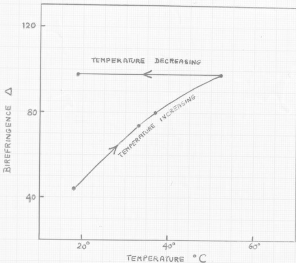
FIG. 2. EFFECT OF TEMPERATURE ON BIREFRINGENCE OF 1.9% BENTONITE SOL WITHOUT ADDED ELECTROLYTE.
