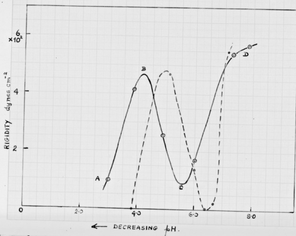
SHOWING EFFECT OF ELECTRODIALYSIS ON RIGIDITY OF BENTONITE.
