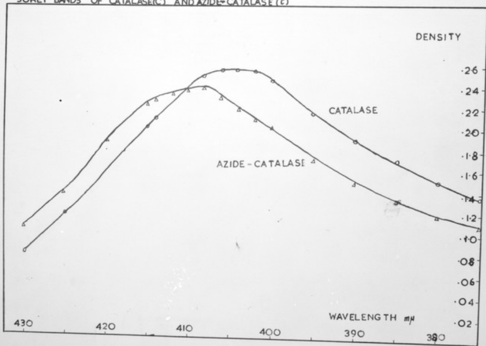
FIG 4 SORET BANDS OF CATALASE(C) AND AZIDE-CATALASE (c)
