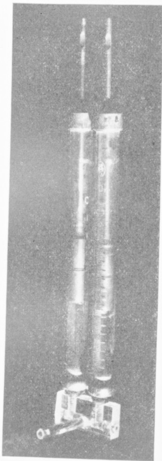
Complete syringe units using two one cc. tuberculin type record syringes.
