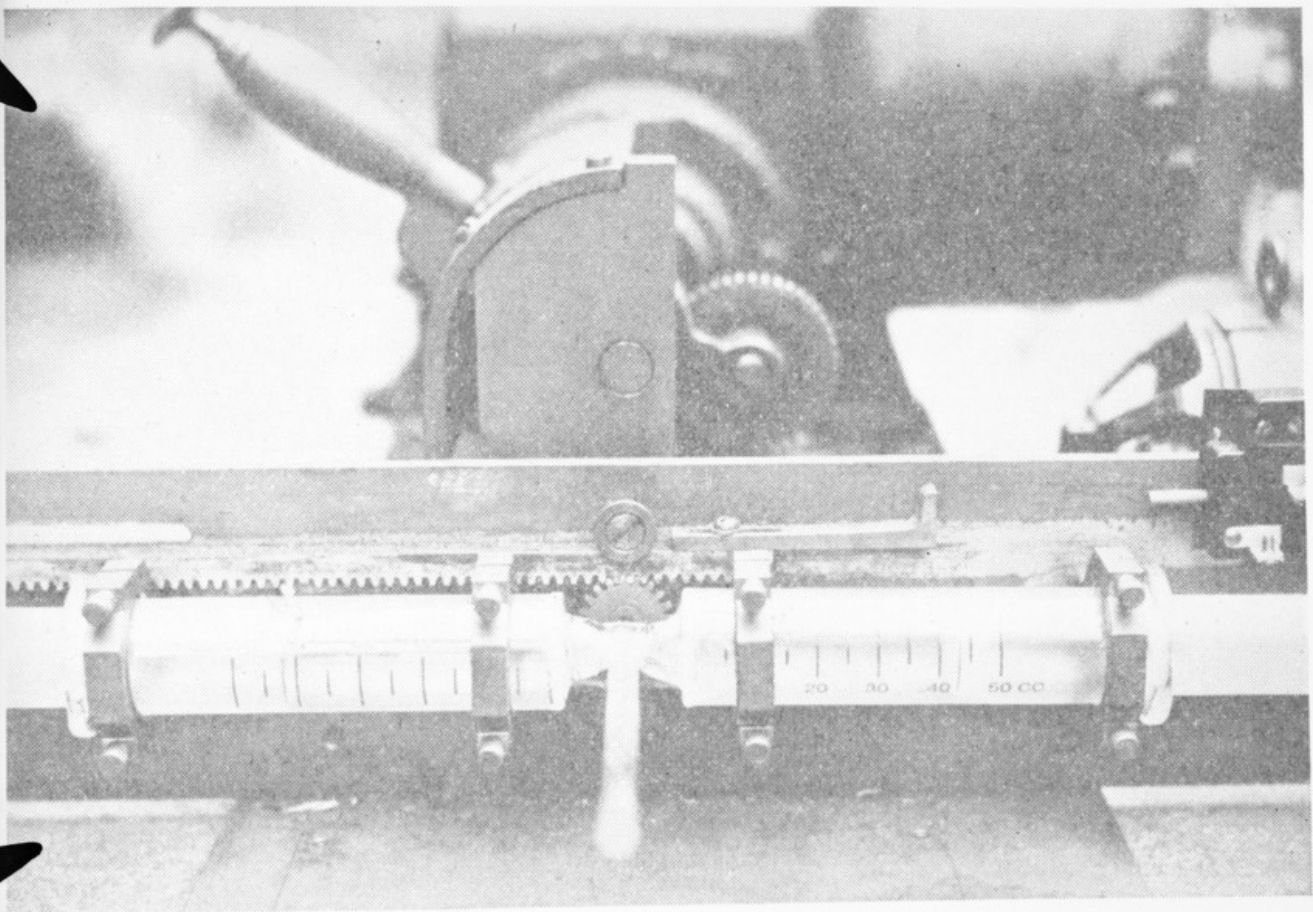
Motor driven syringe unit with horizontal opposed all glass syringe unit and belted generator for flow base.
