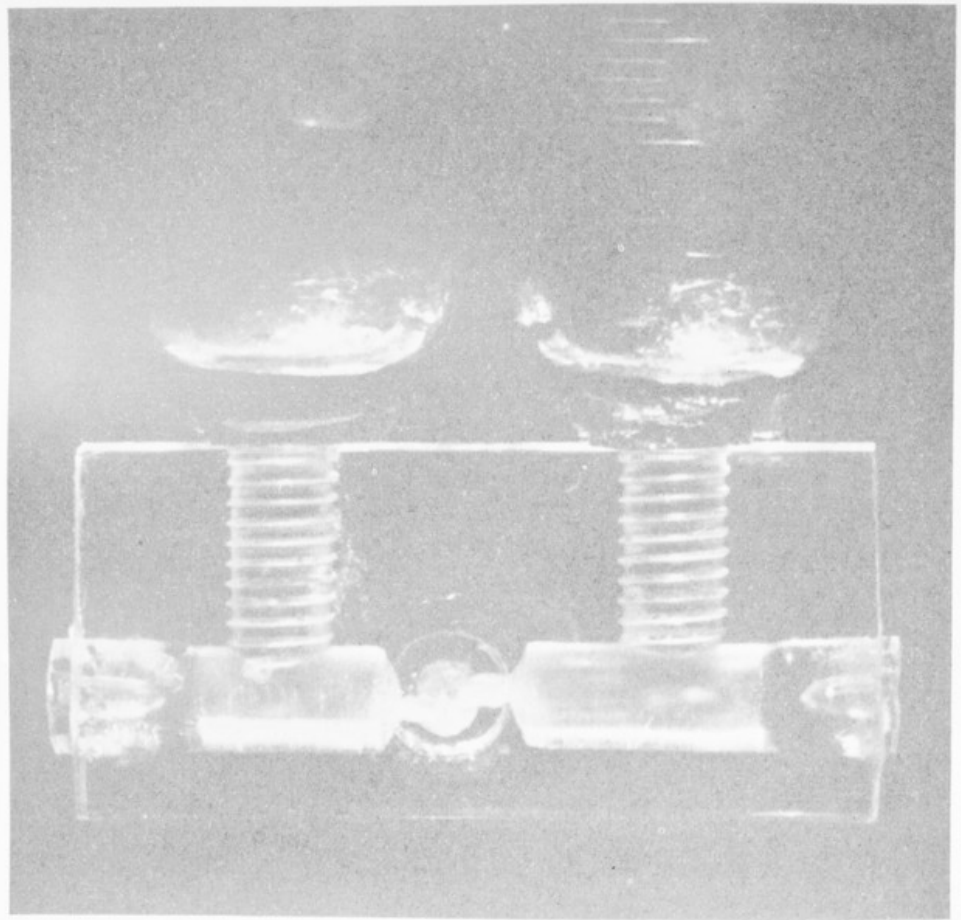
Lucite mixing chamber showing tangential jets and rear of observation tube seal.
