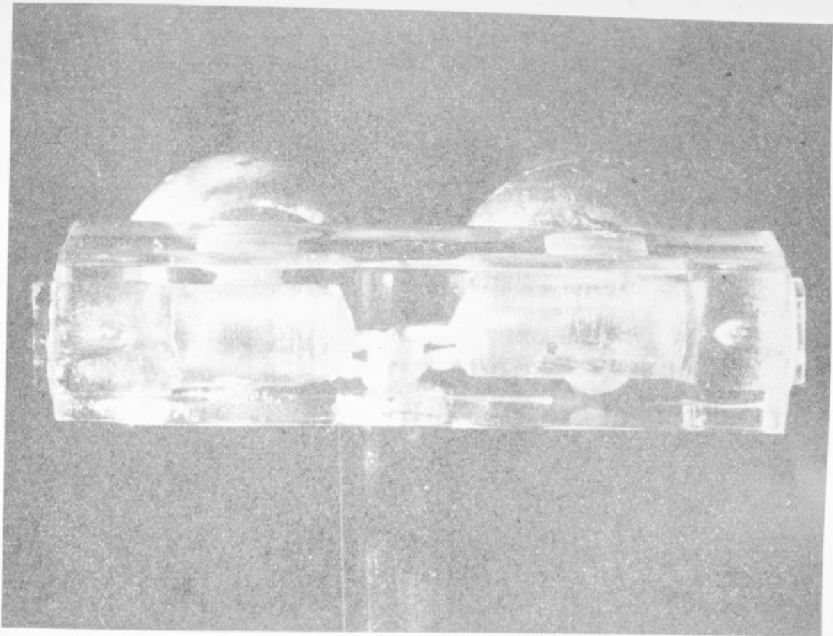
Lucite mixing chamber showing double jet arrangement, observation tube seal, and glass observation tube.
